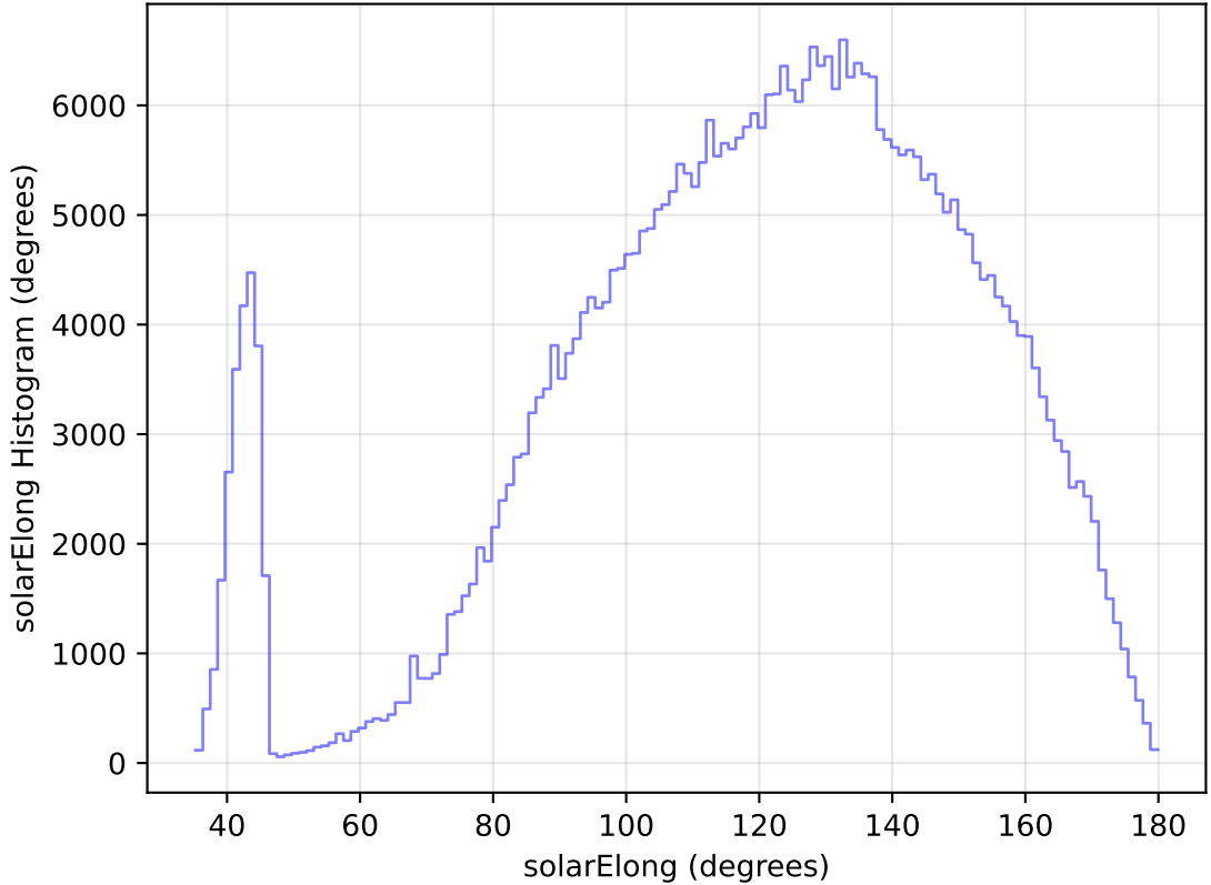
internal_u_expt38_nscale0.9v3.4_10yrs All sky z band: solarElong Histogram
