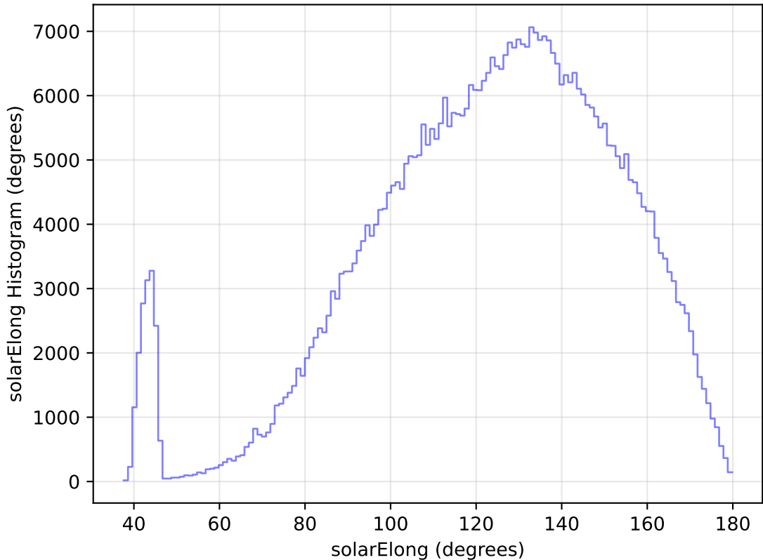
internal_u_expt38_nscale0.9v3.4_10yrs All sky r band: solarElong Histogram
