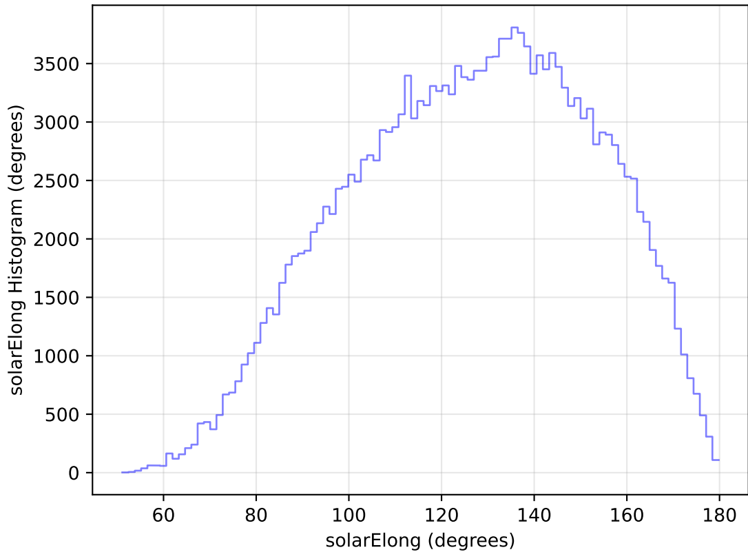
internal_u_expt38_nscale0.9v3.4_10yrs All sky g band: solarElong Histogram
