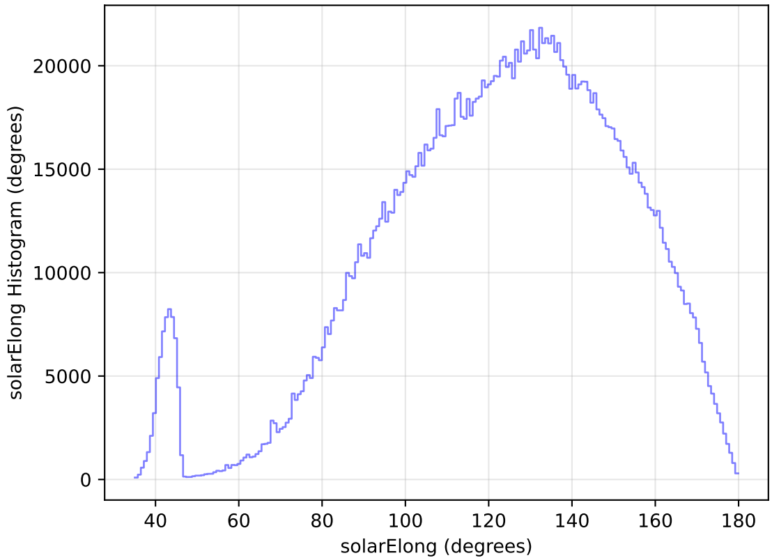
internal_u_expt38_nscale0.9v3.4_10yrs All sky all bands: solarElong Histogram
