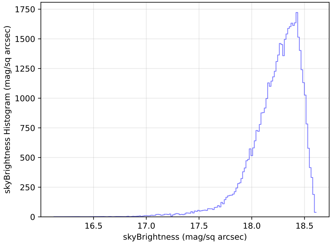
internal_u_expt38_nscale0.9v3.4_10yrs Yr 1 y band: skyBrightness Histogram
