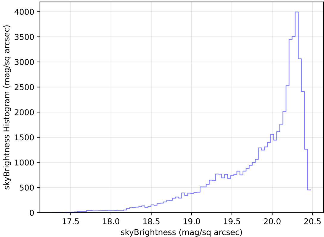
internal_u_expt38_nscale0.9v3.4_10yrs Yr 1 i band: skyBrightness Histogram
