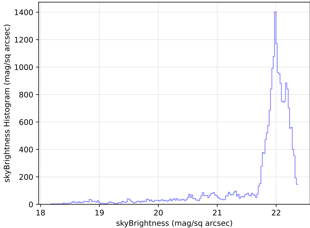
internal_u_expt38_nscale0.9v3.4_10yrs Yr 1 g band: skyBrightness Histogram
