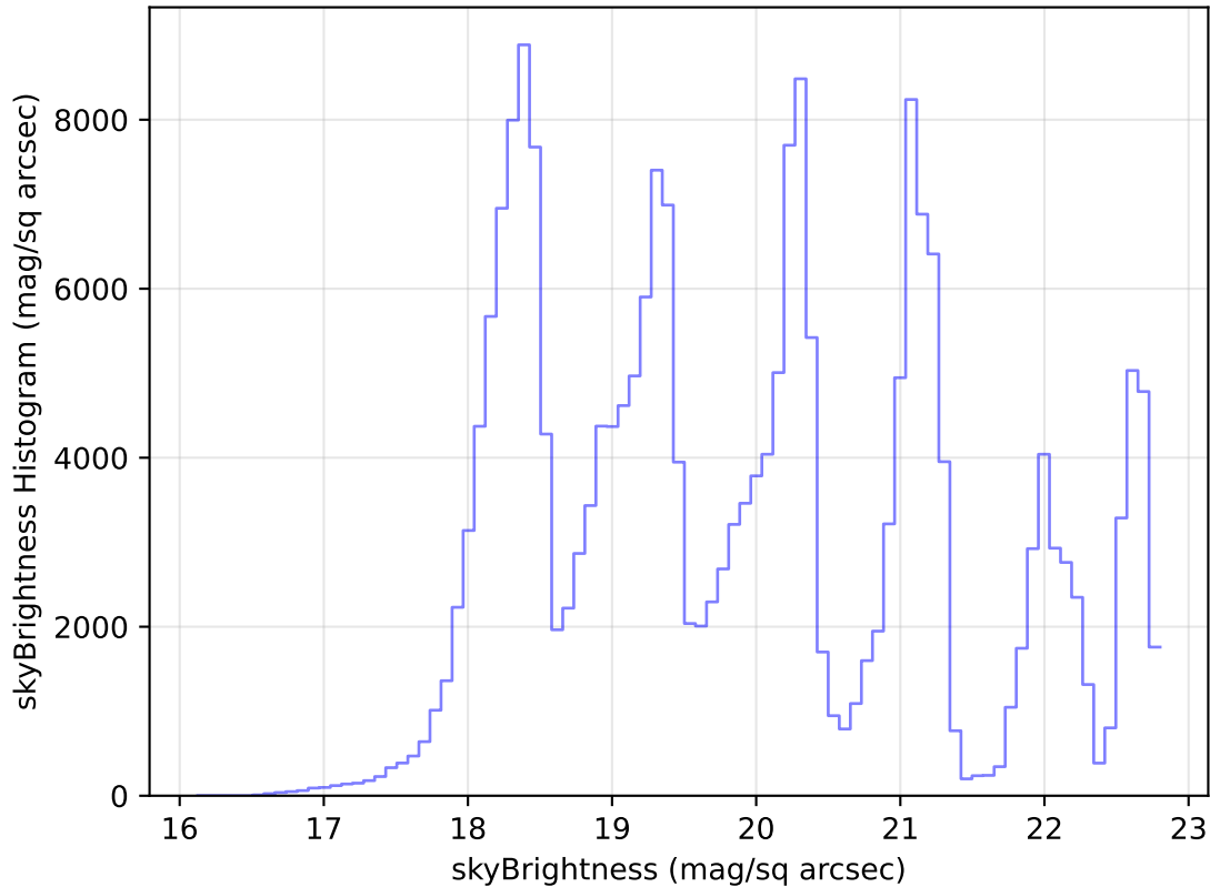
internal_u_expt38_nscale0.9v3.4_10yrs Yr 1 all bands: skyBrightness Histogram
