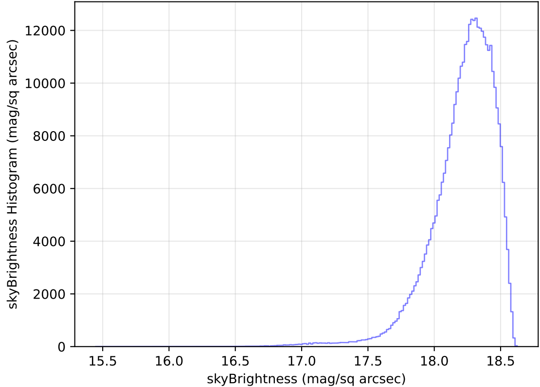
internal_u_expt38_nscale0.9v3.4_10yrs WFD y band: skyBrightness Histogram
