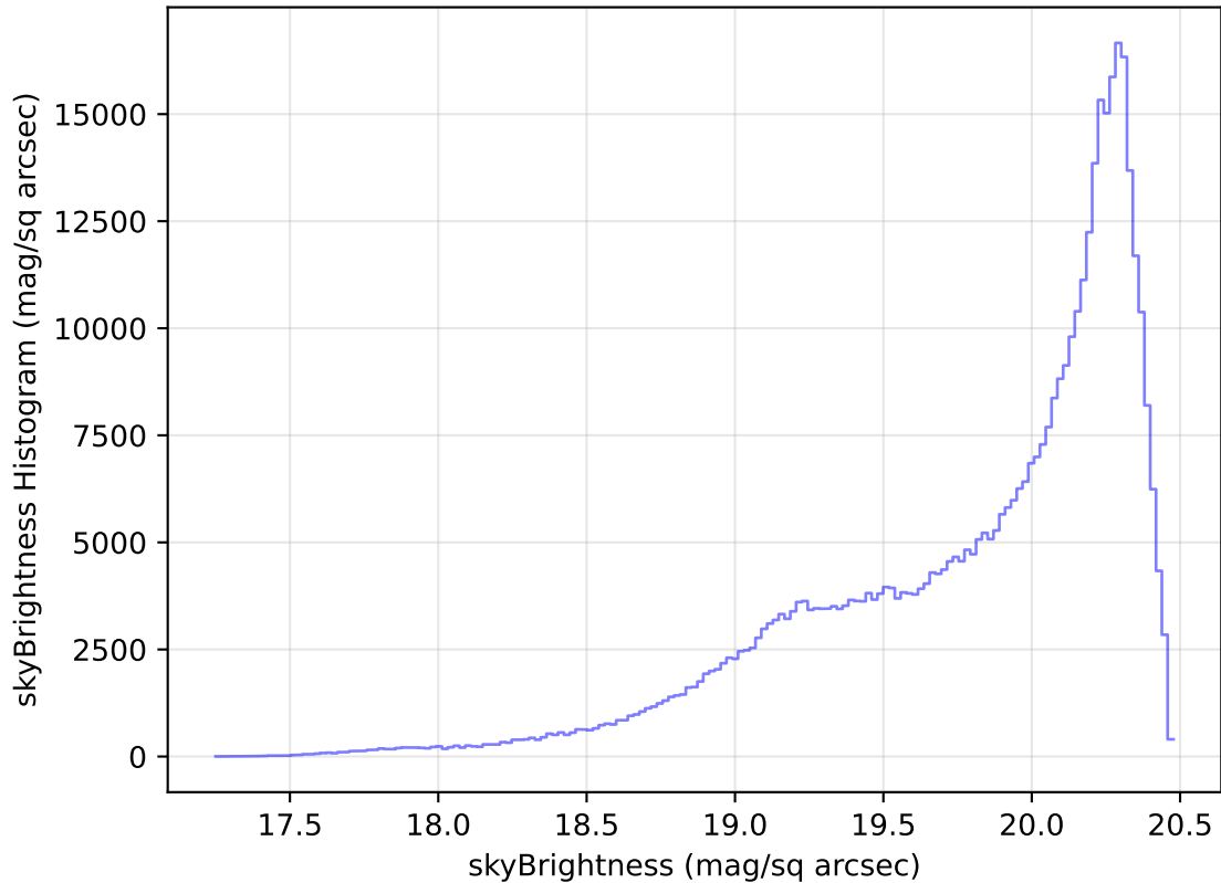
internal_u_expt38_nscale0.9v3.4_10yrs WFD i band: skyBrightness Histogram
