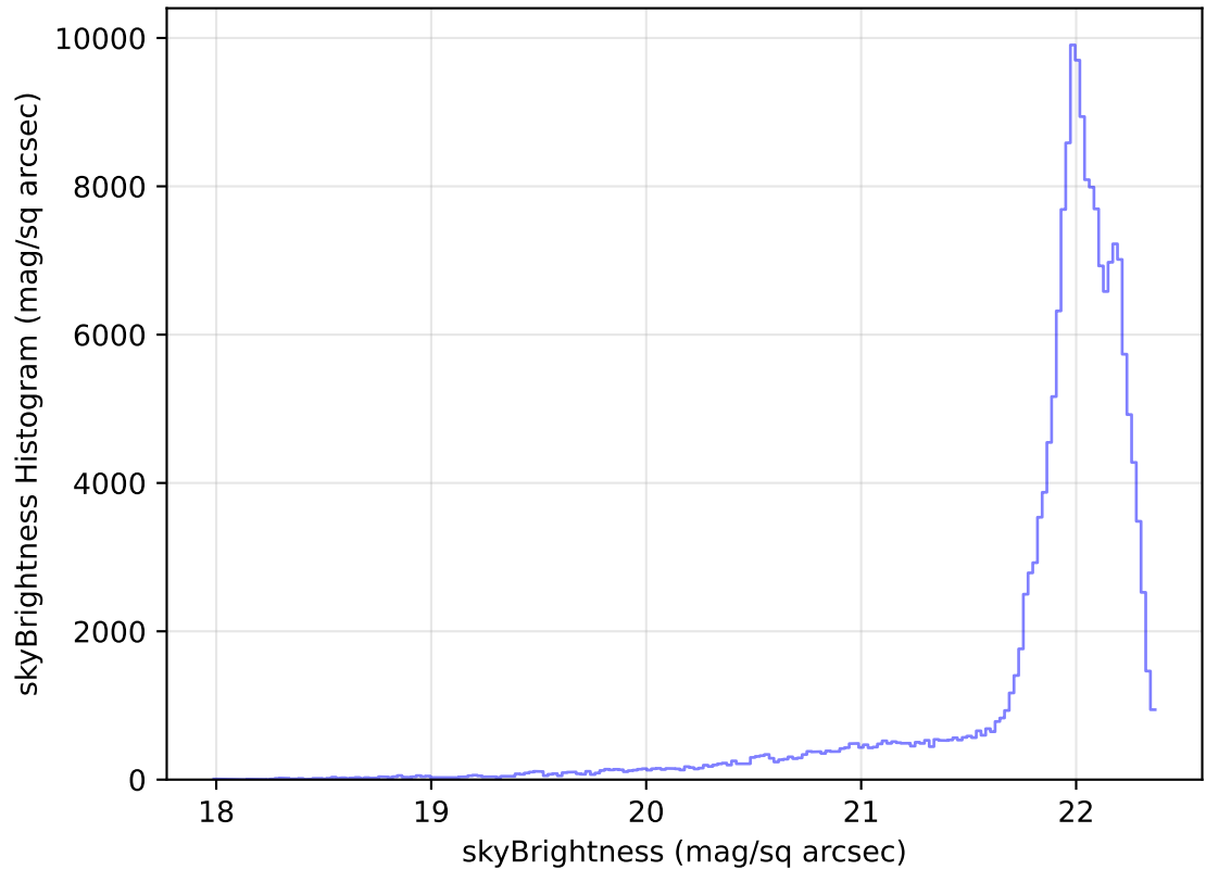
internal_u_expt38_nscale0.9v3.4_10yrs WFD g band: skyBrightness Histogram
