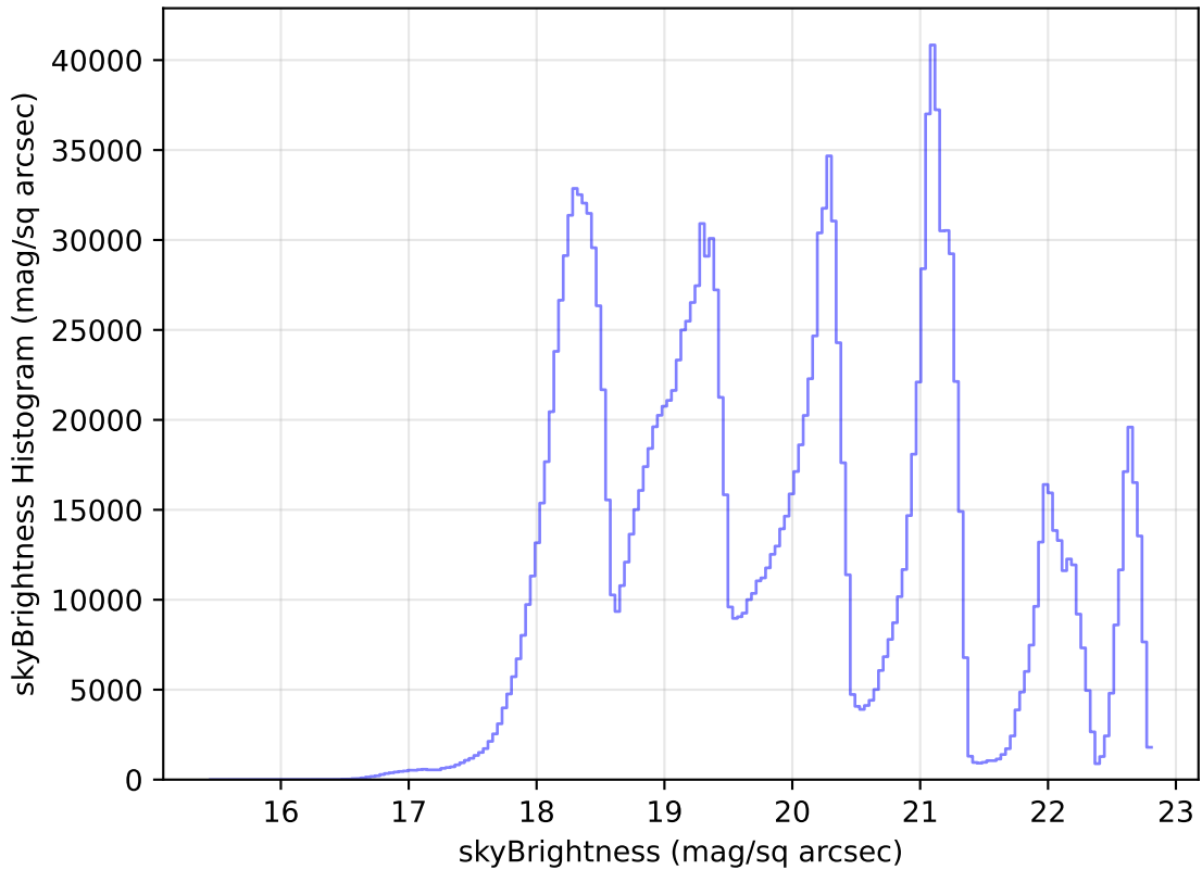
internal_u_expt38_nscale0.9v3.4_10yrs WFD all bands: skyBrightness Histogram
