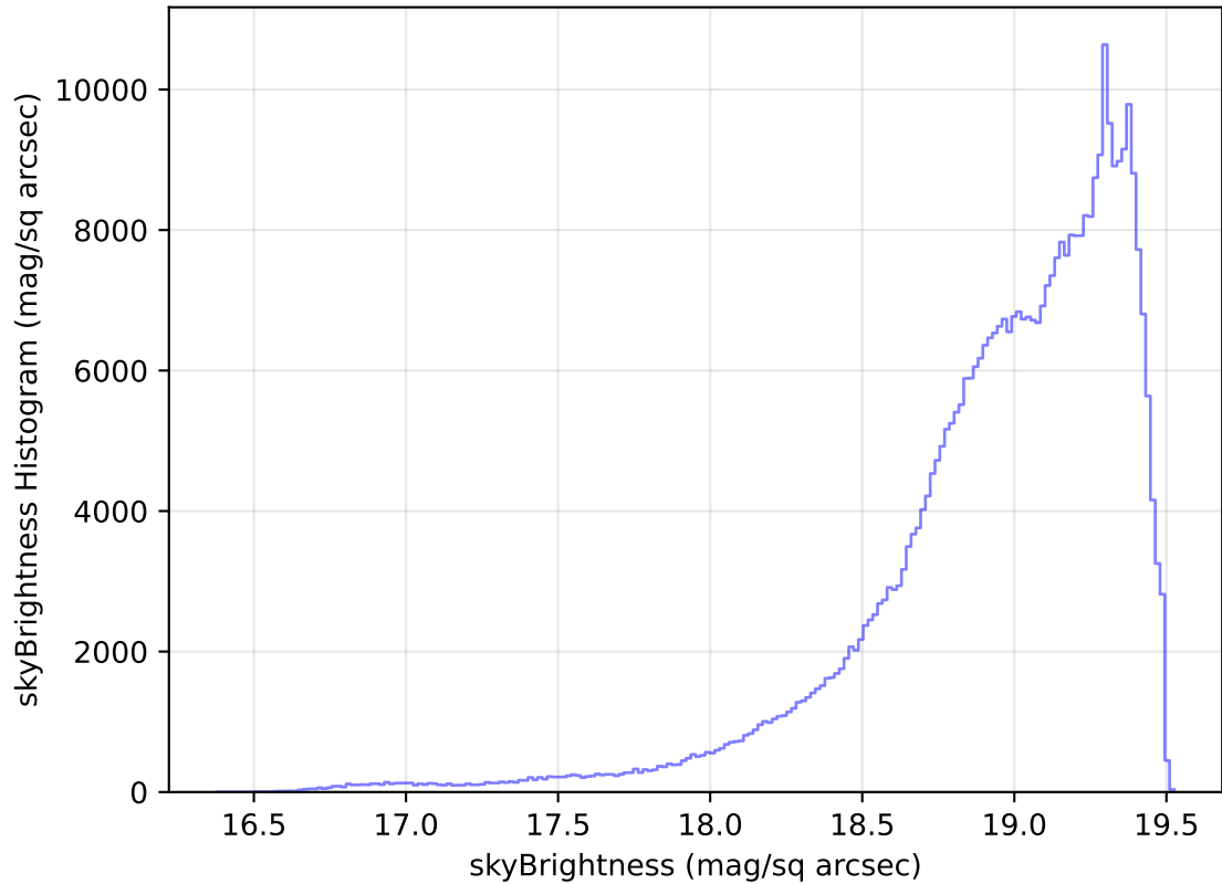
internal_u_expt38_nscale0.9v3.4_10yrs All sky z band: skyBrightness Histogram
