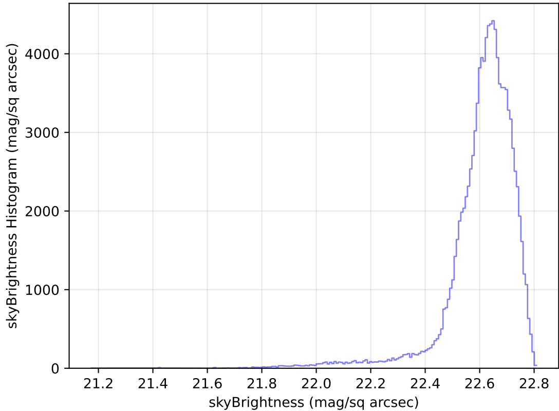
internal_u_expt38_nscale0.9v3.4_10yrs All sky u band: skyBrightness Histogram
