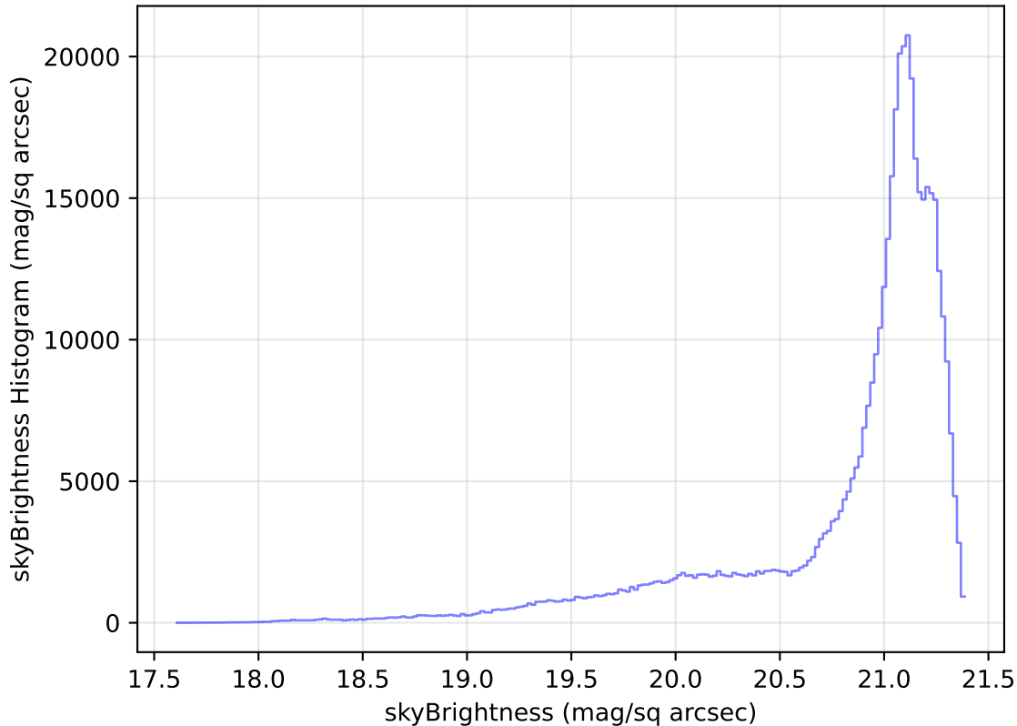
internal_u_expt38_nscale0.9v3.4_10yrs All sky r band: skyBrightness Histogram
