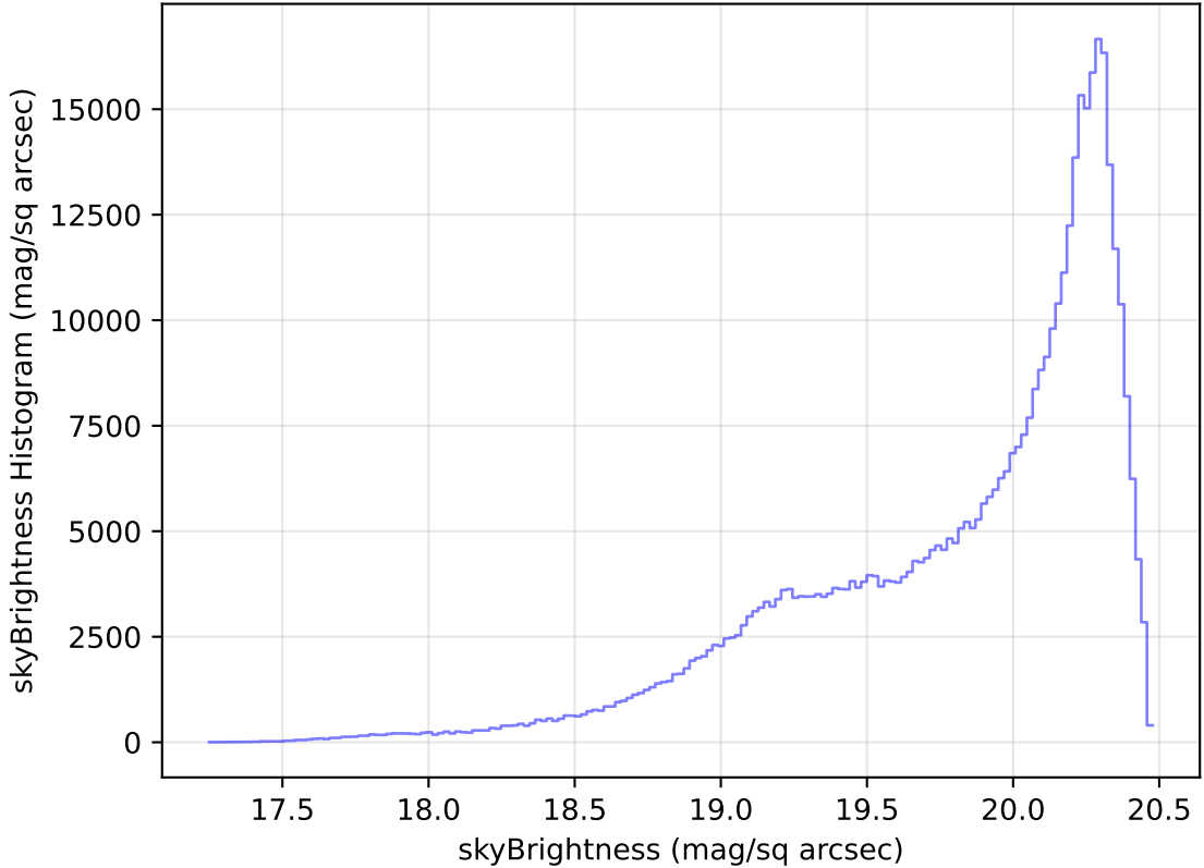
internal_u_expt38_nscale0.9v3.4_10yrs All sky i band: skyBrightness Histogram
