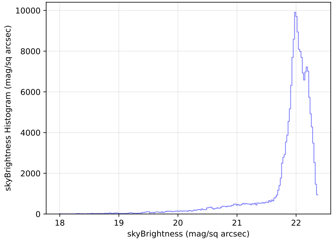
internal_u_expt38_nscale0.9v3.4_10yrs All sky g band: skyBrightness Histogram
