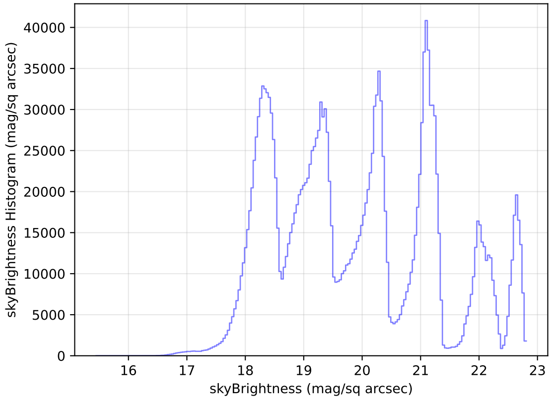
internal_u_expt38_nscale0.9v3.4_10yrs All sky all bands: skyBrightness Histogram
