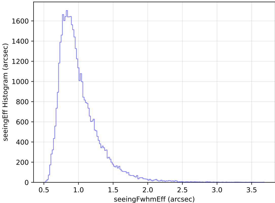
internal_u_expt38_nscale0.9v3.4_10yrs Yr 1 z band: seeingEff Histogram
