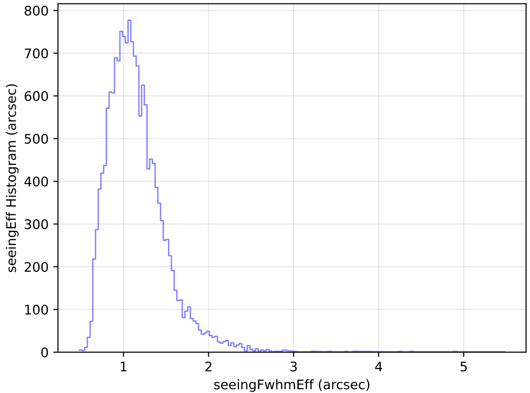
internal_u_expt38_nscale0.9v3.4_10yrs Yr 1 u band: seeingEff Histogram
