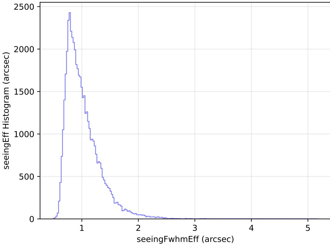
internal_u_expt38_nscale0.9v3.4_10yrs Yr 1 r band: seeingEff Histogram
