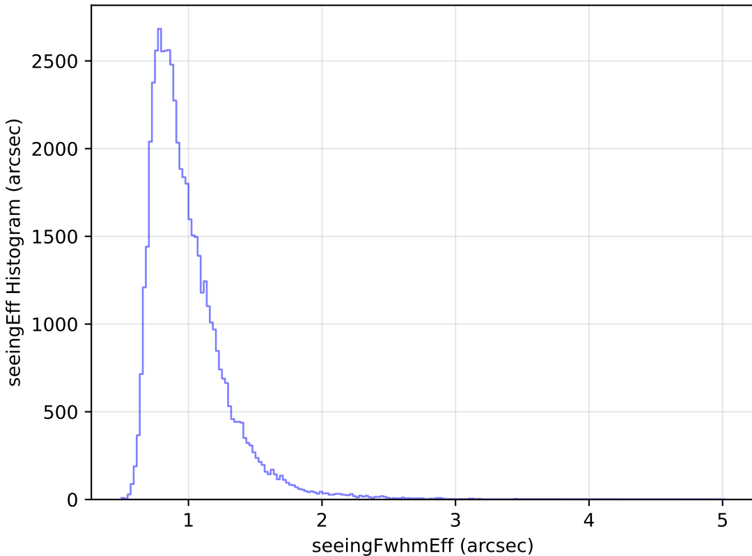
internal_u_expt38_nscale0.9v3.4_10yrs Yr 1 i band: seeingEff Histogram
