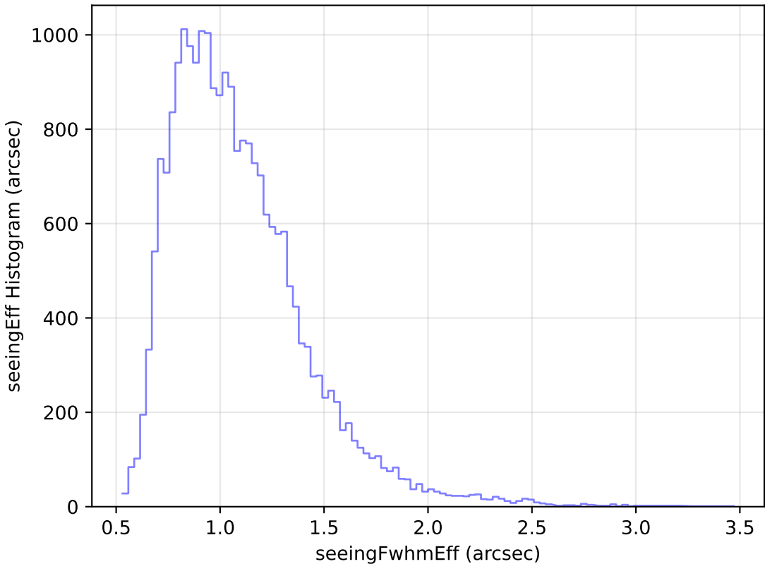
internal_u_expt38_nscale0.9v3.4_10yrs Yr 1 g band: seeingEff Histogram
