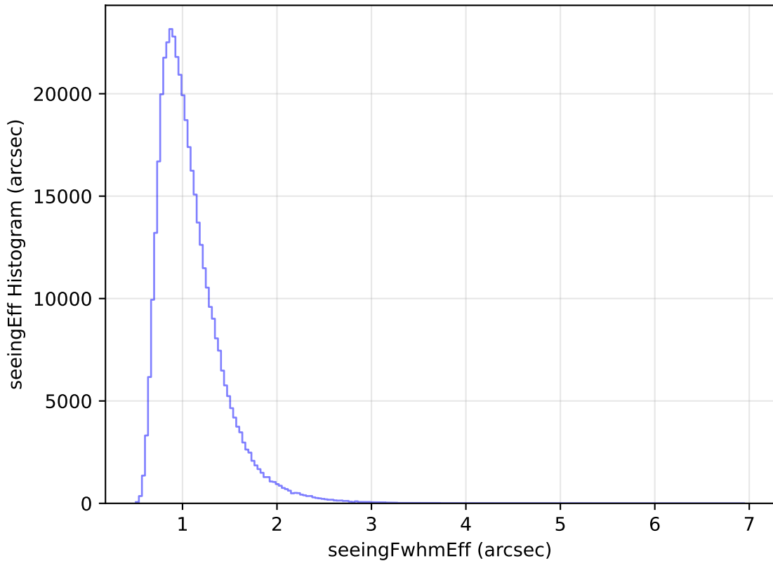
internal_u_expt38_nscale0.9v3.4_10yrs WFD z band: seeingEff Histogram
