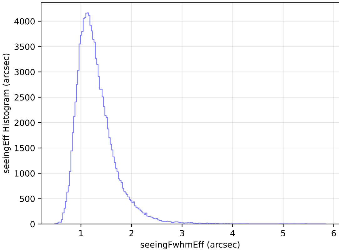
internal_u_expt38_nscale0.9v3.4_10yrs WFD u band: seeingEff Histogram
