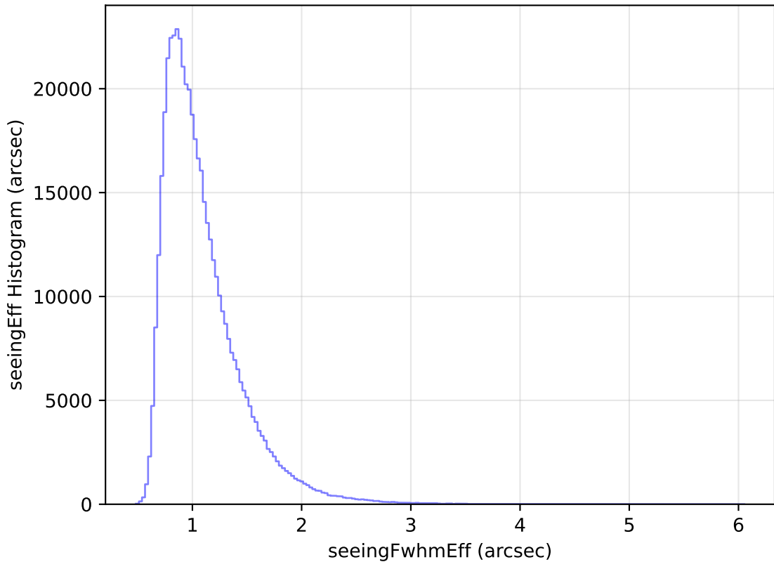
internal_u_expt38_nscale0.9v3.4_10yrs WFD i band: seeingEff Histogram
