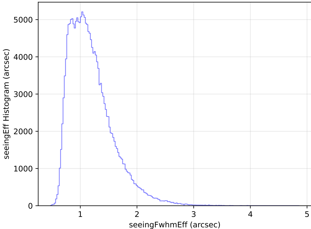
internal_u_expt38_nscale0.9v3.4_10yrs WFD g band: seeingEff Histogram
