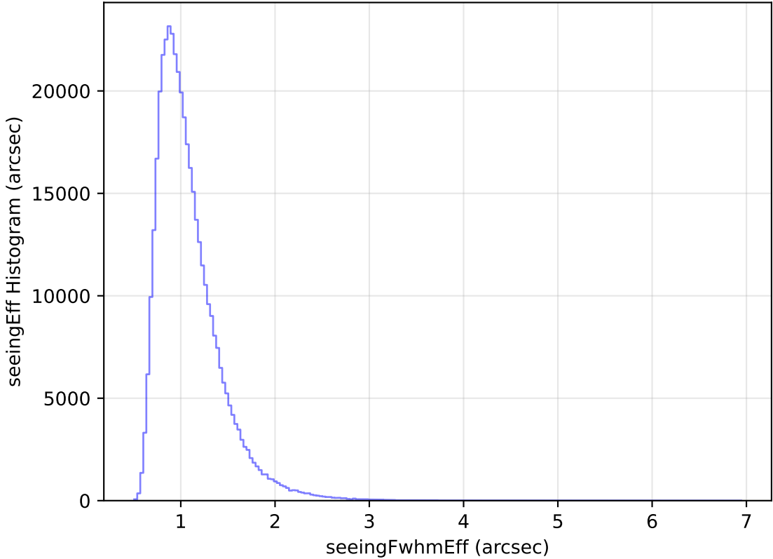
internal_u_expt38_nscale0.9v3.4_10yrs All sky z band: seeingEff Histogram
