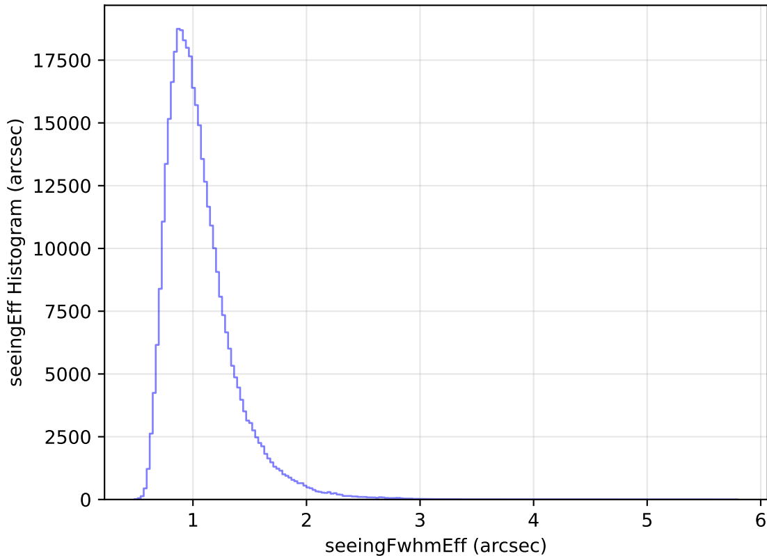
internal_u_expt38_nscale0.9v3.4_10yrs All sky y band: seeingEff Histogram
