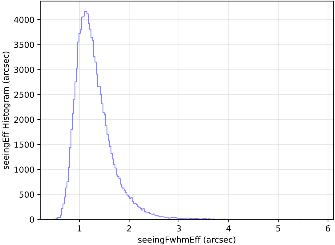
internal_u_expt38_nscale0.9v3.4_10yrs All sky u band: seeingEff Histogram
