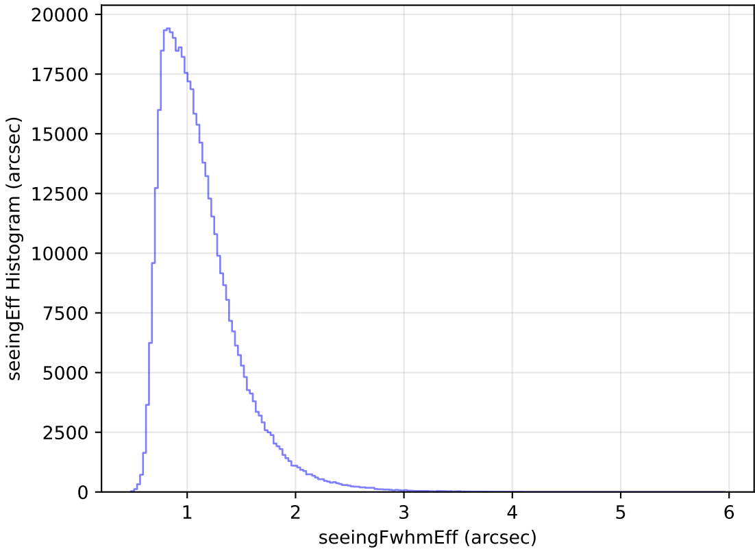
internal_u_expt38_nscale0.9v3.4_10yrs All sky r band: seeingEff Histogram
