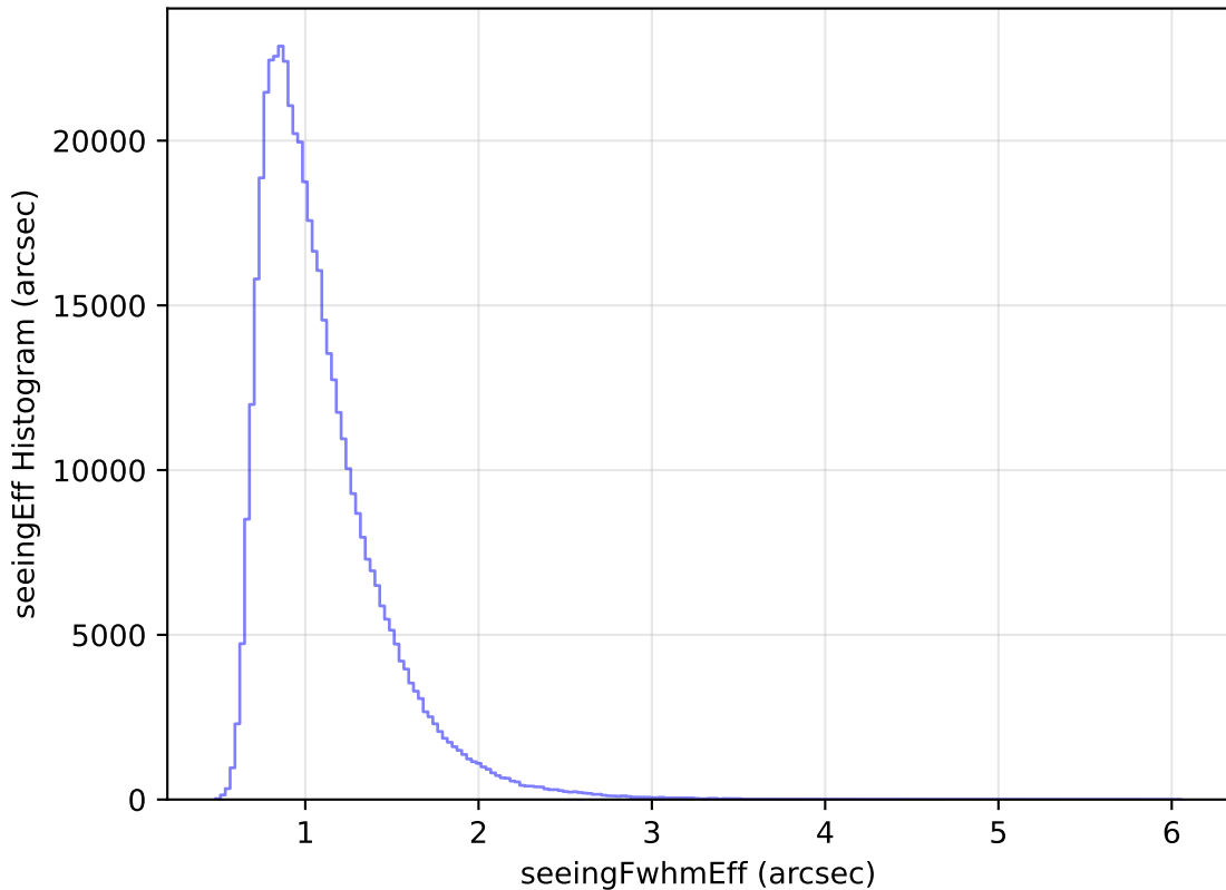
internal_u_expt38_nscale0.9v3.4_10yrs All sky i band: seeingEff Histogram
