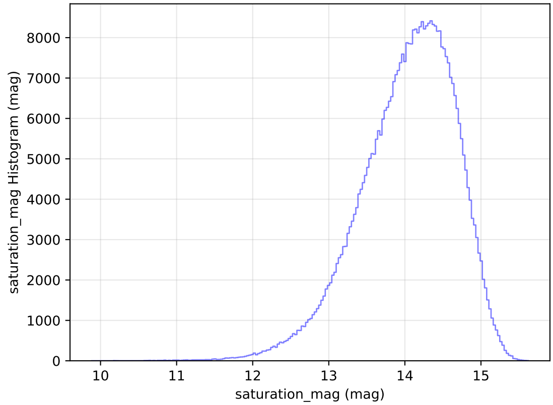
internal_u_expt38_nscale0.9v3.4_10yrs WFD z band: saturation_mag Histogram
