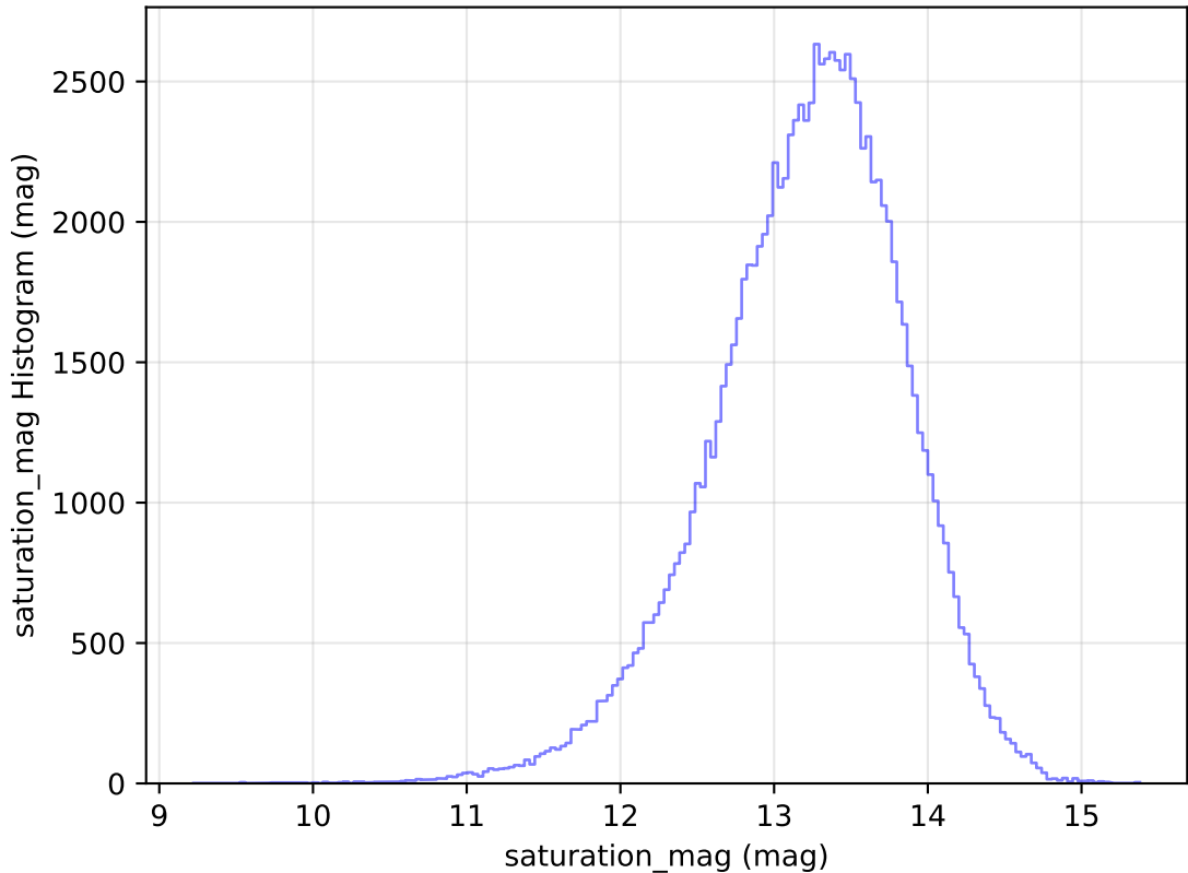
internal_u_expt38_nscale0.9v3.4_10yrs WFD u band: saturation_mag Histogram
