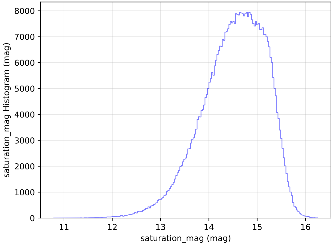
internal_u_expt38_nscale0.9v3.4_10yrs WFD r band: saturation_mag Histogram
