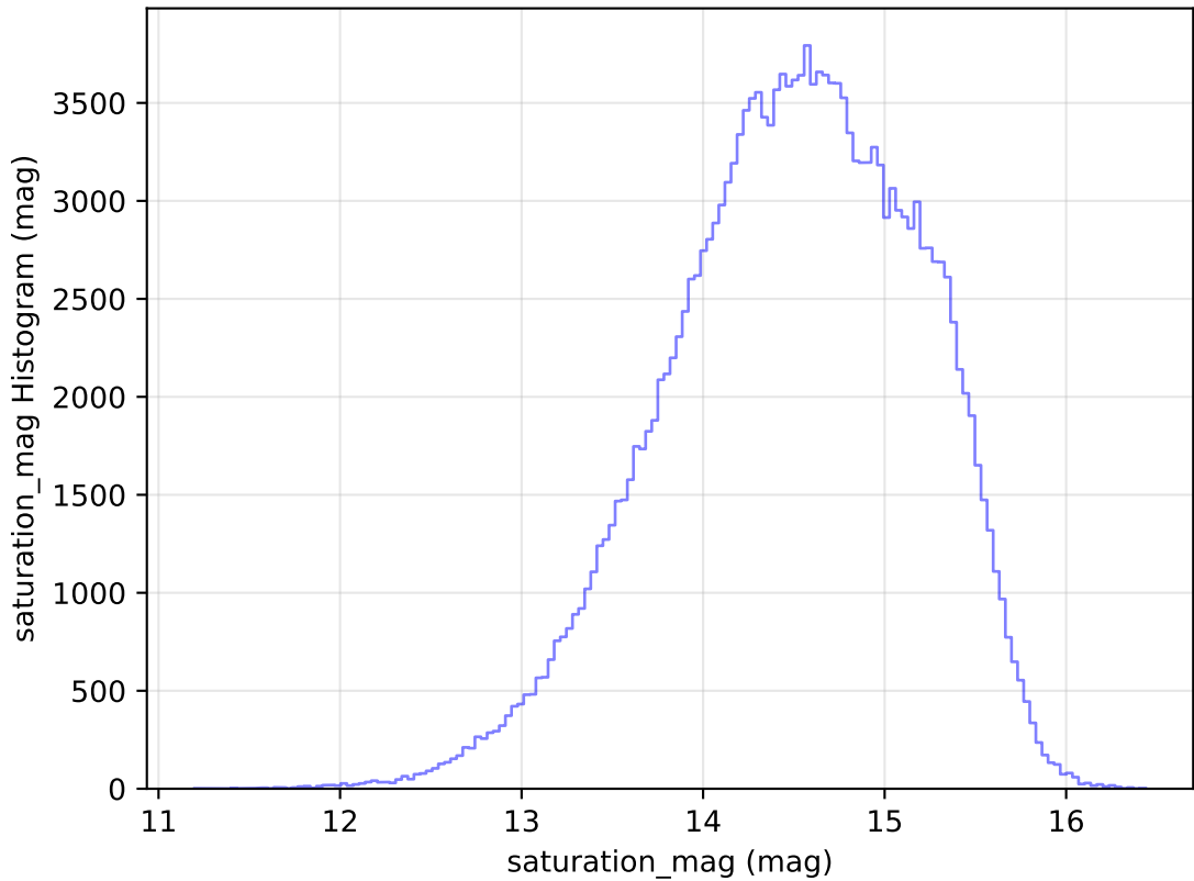
internal_u_expt38_nscale0.9v3.4_10yrs WFD g band: saturation_mag Histogram
