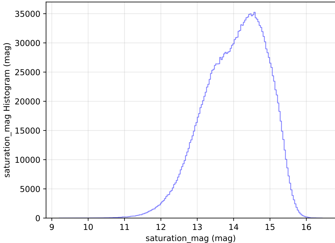
internal_u_expt38_nscale0.9v3.4_10yrs WFD all bands: saturation_mag Histogram
