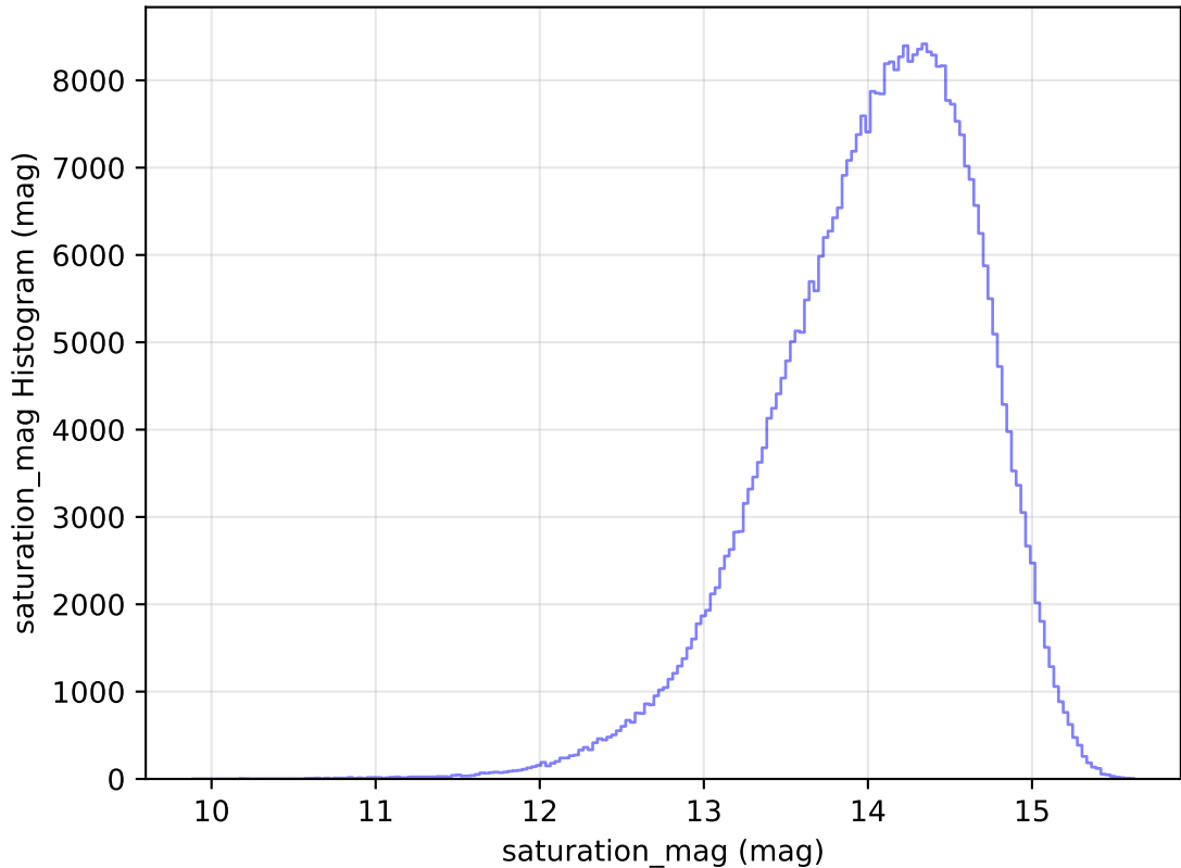
internal_u_expt38_nscale0.9v3.4_10yrs All sky z band: saturation_mag Histogram
