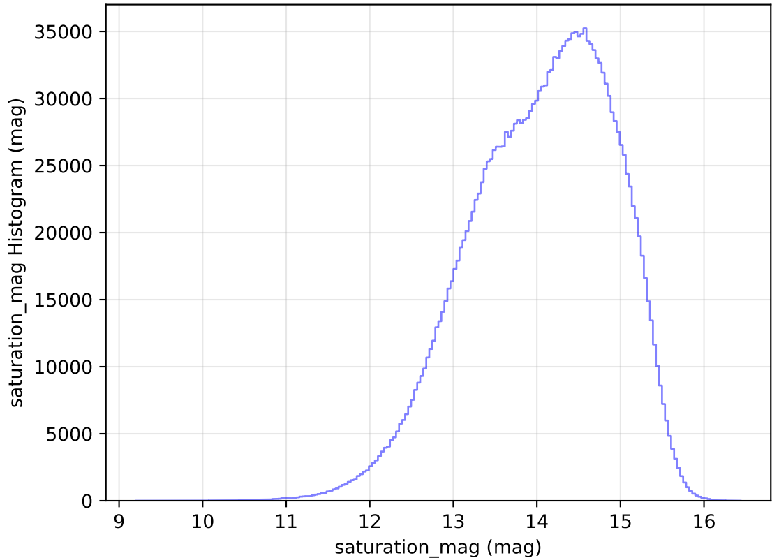
internal_u_expt38_nscale0.9v3.4_10yrs All sky all bands: saturation_mag Histogram
