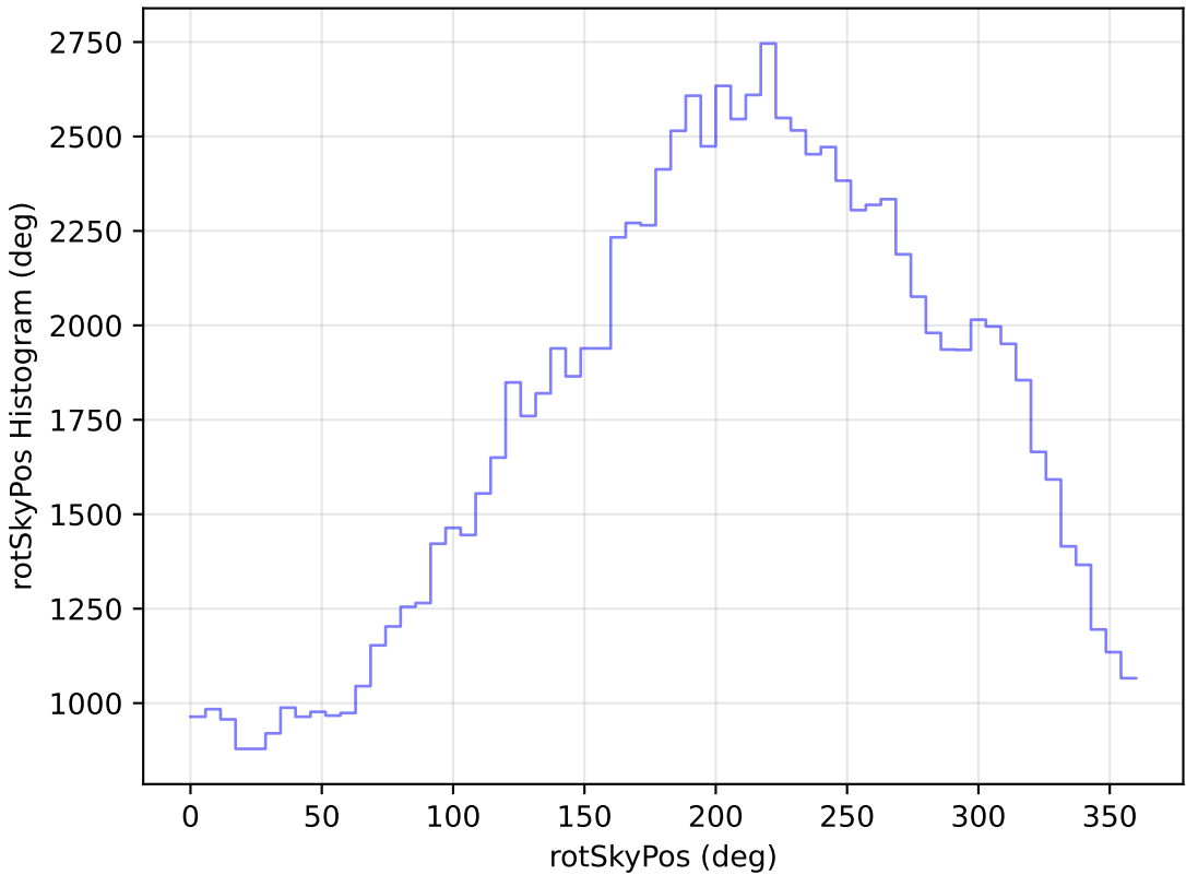
internal_u_expt38_nscale0.9v3.4_10yrs WFD u band: rotSkyPos Histogram
