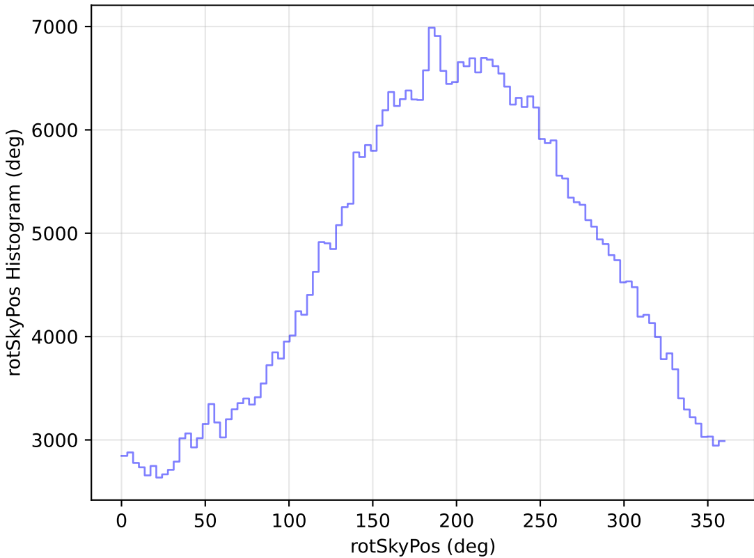
internal_u_expt38_nscale0.9v3.4_10yrs WFD r band: rotSkyPos Histogram
