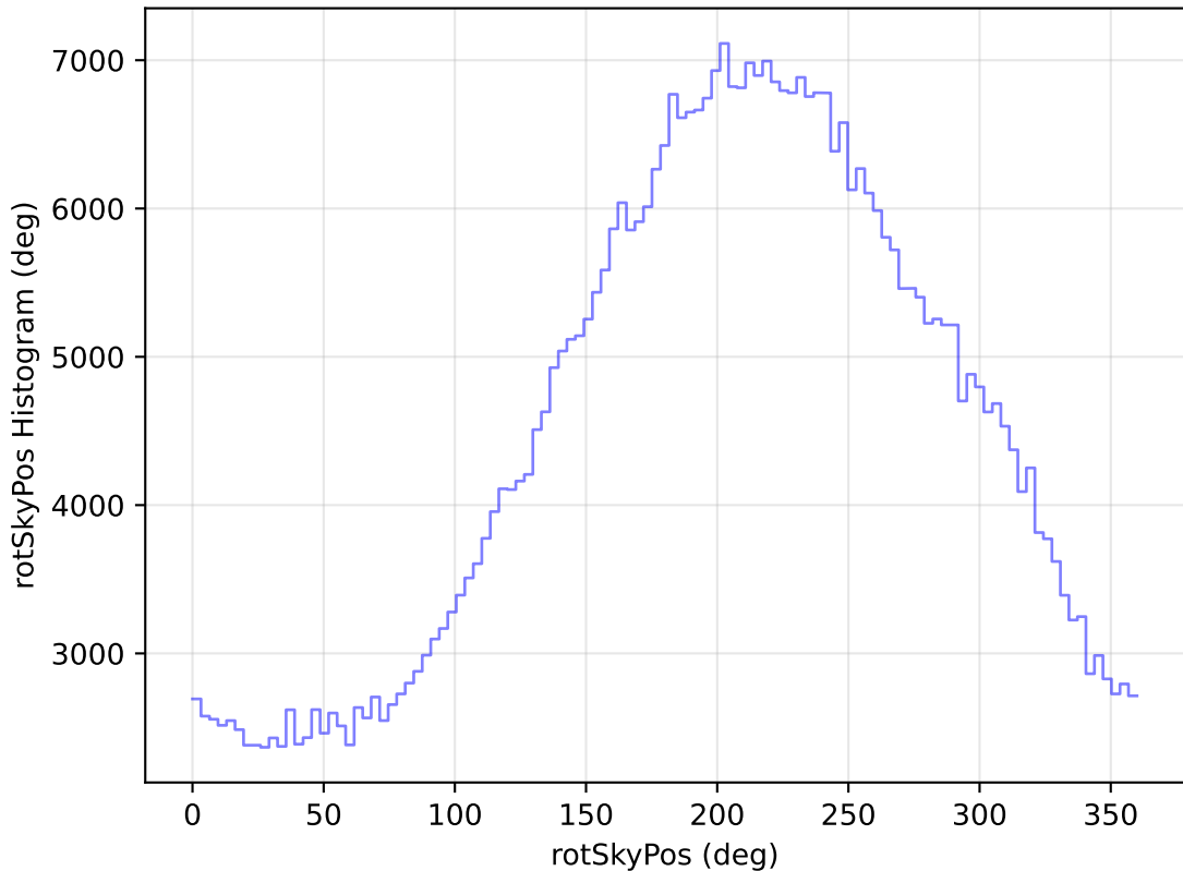
internal_u_expt38_nscale0.9v3.4_10yrs WFD i band: rotSkyPos Histogram
