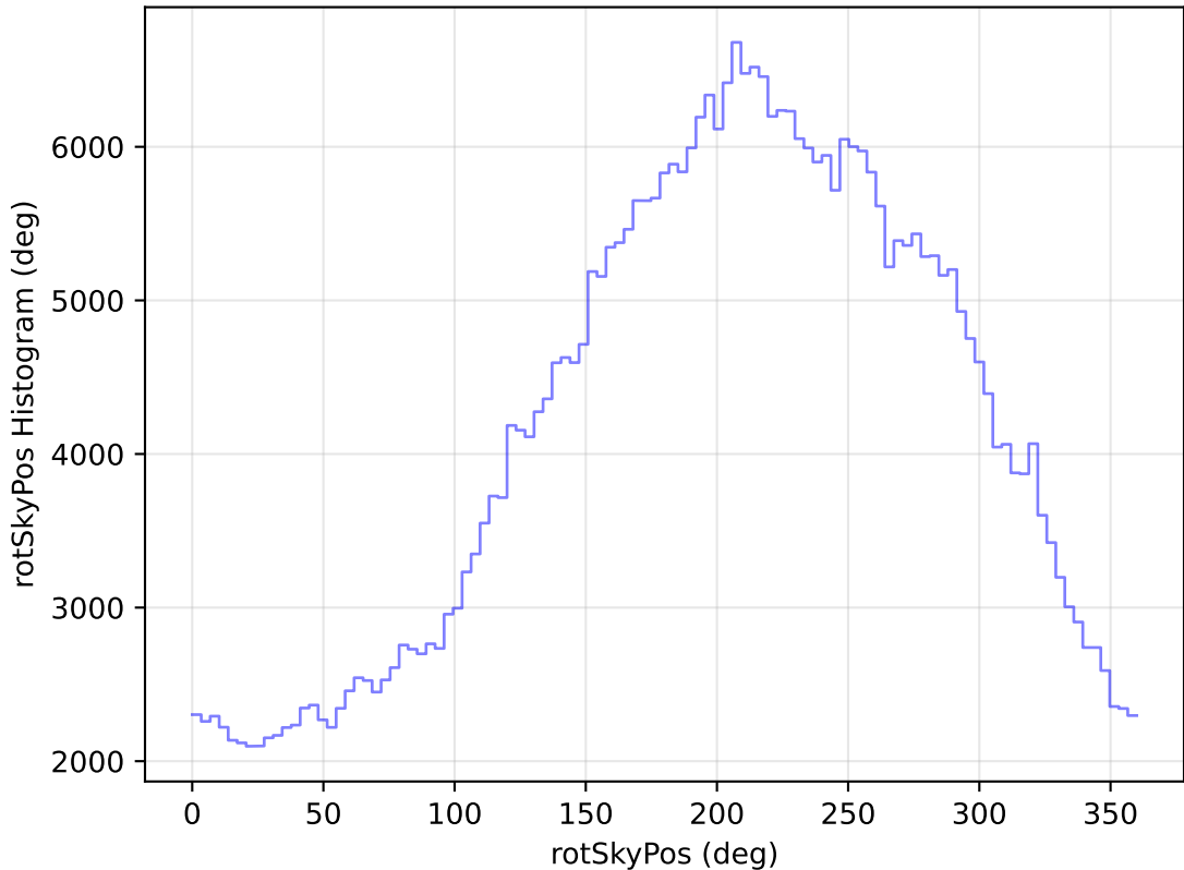
internal_u_expt38_nscale0.9v3.4_10yrs All sky z band: rotSkyPos Histogram
