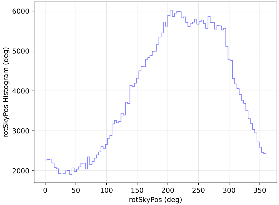
internal_u_expt38_nscale0.9v3.4_10yrs All sky y band: rotSkyPos Histogram
