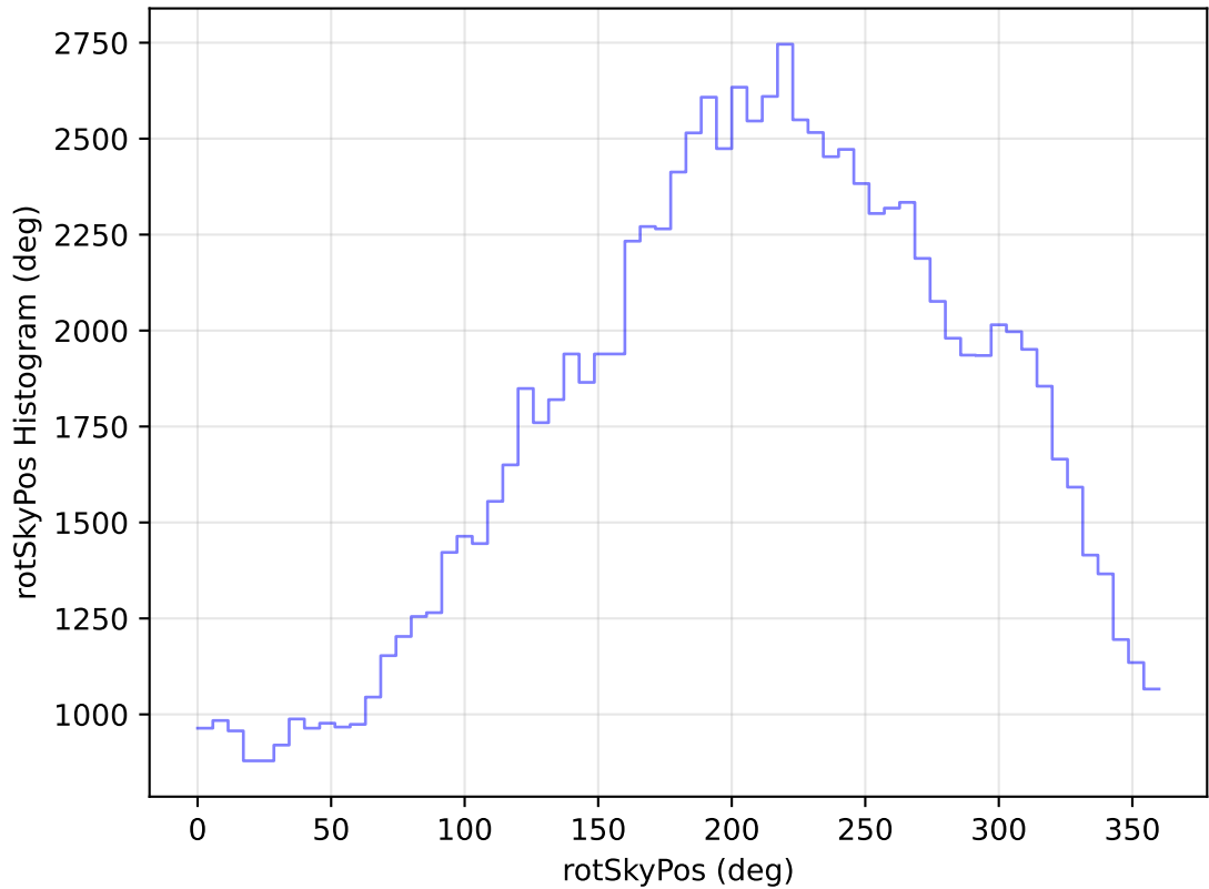
internal_u_expt38_nscale0.9v3.4_10yrs All sky u band: rotSkyPos Histogram
