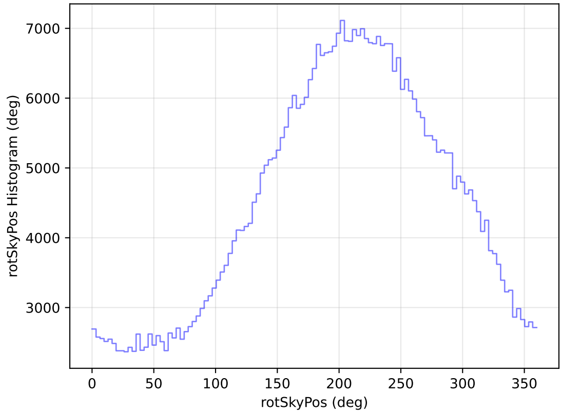
internal_u_expt38_nscale0.9v3.4_10yrs All sky i band: rotSkyPos Histogram
