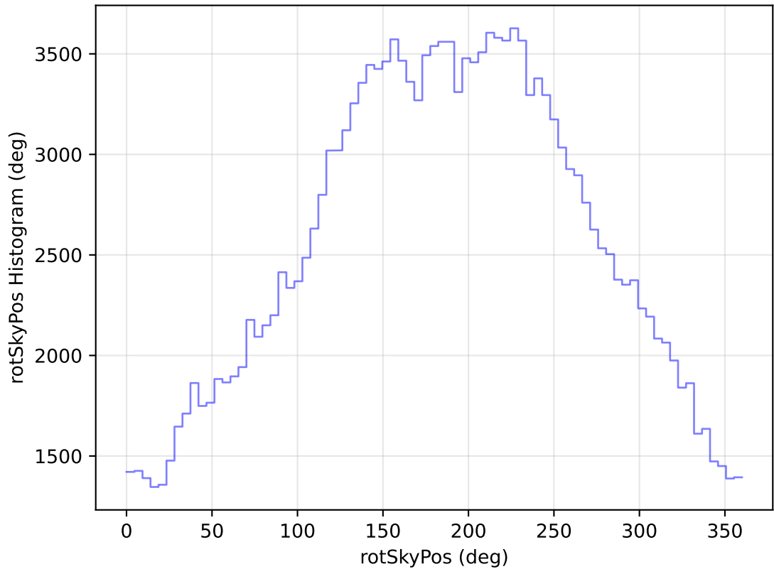
internal_u_expt38_nscale0.9v3.4_10yrs All sky g band: rotSkyPos Histogram
