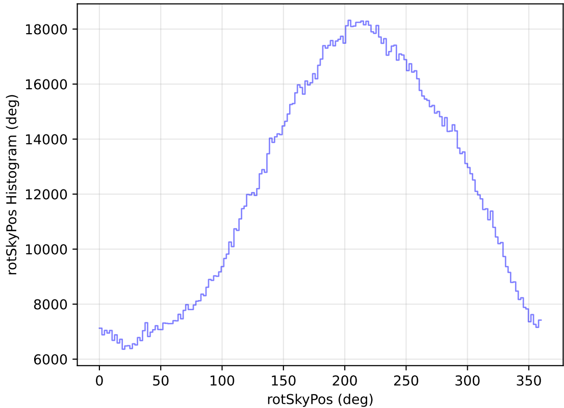
internal_u_expt38_nscale0.9v3.4_10yrs All sky all bands: rotSkyPos Histogram
