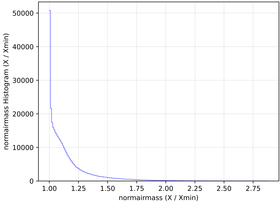
internal_u_expt38_nscale0.9v3.4_10yrs WFD y band: normairmass Histogram
