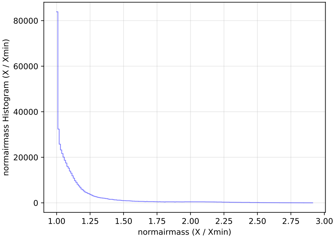
internal_u_expt38_nscale0.9v3.4_10yrs WFD i band: normairmass Histogram
